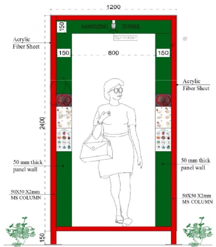
SANITIZING TUNNEL ELEVATION-A
