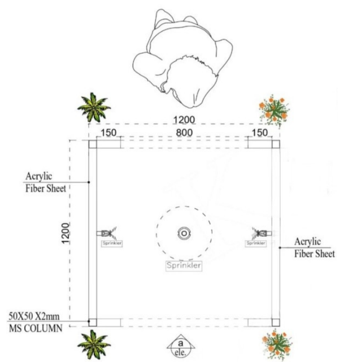
4'-0" X 4'-0" SANITIZING TUNNEL LAYOUT DRAWING
