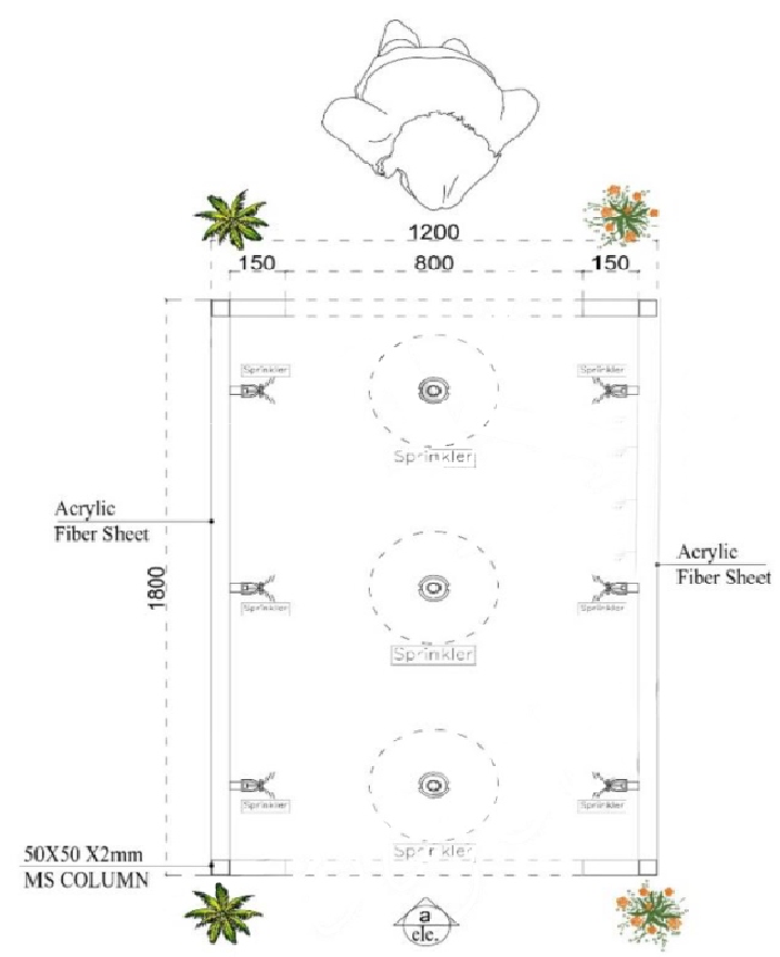
4'-0" X 6'-0" SANITIZING TUNNEL LAYOUT DRAWING
